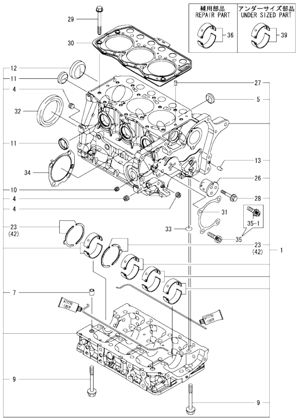
Fig.1. CYLINDER BLOCK
